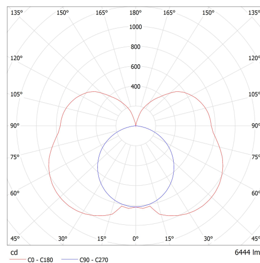
Luminaire: Lucis ZLI3.L2.1500.X IZAR III LED Lamps: 1 x LED G6
