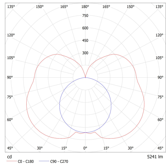
Luminaire: Lucis I3.L1.1200.X IZAR III LED Lamps: 1 x LED G6
