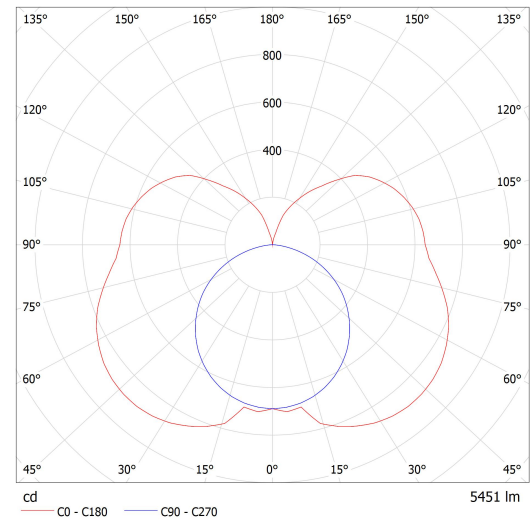
Luminaire: Lucis I3.L2.1200.X IZAR III LED Lamps: 1 x LED G6
