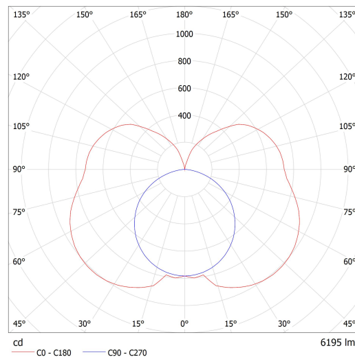
Luminaire: Lucis I3.L1.1500.X IZAR III LED Lamps: 1 x LED G6
