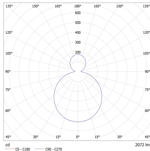
Luminaire: Lucis PS13.K1.R450 RONDO LED Lamps: 1 x LED G5
