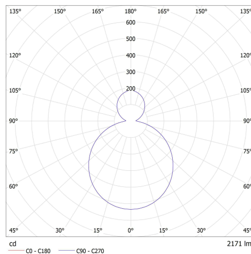
Lucis PS13.K2.R450 RONDO LED / LDC (Polar)
