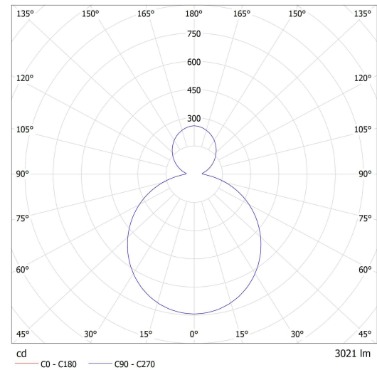
Lucis PS13.K1.R550 RONDO LED / LDC (Polar)
