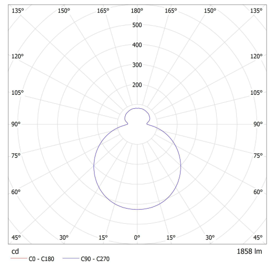
Lucis PS13.K1.Z330 ZERO LED / LDC (Polar)
