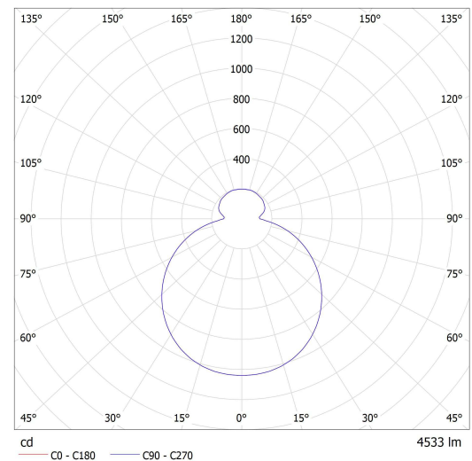
Lucis PS13.K1.Z500 ZERO LED / LDC (Polar)
